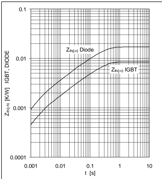
Fig. 16 Thermal impedance vs time
