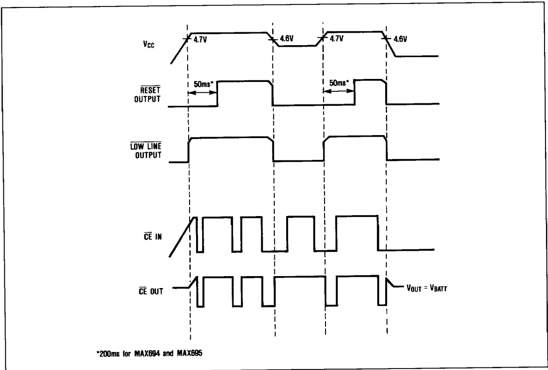
Figure 6. Reset Timing
