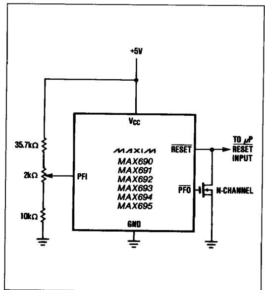
Figure 10. Reset on Overvoltage or Undervoltage
