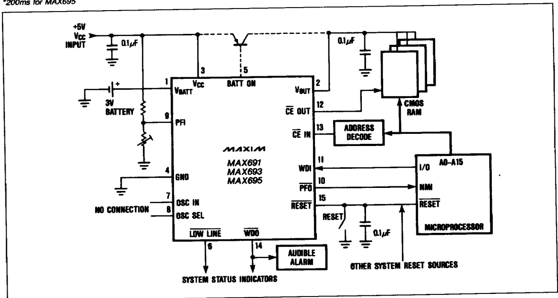
Figure 1. MAX691/693/695 Typical Application
