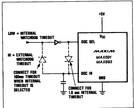
Figure 14. Selecting Internal or External Watchdog Timeout
