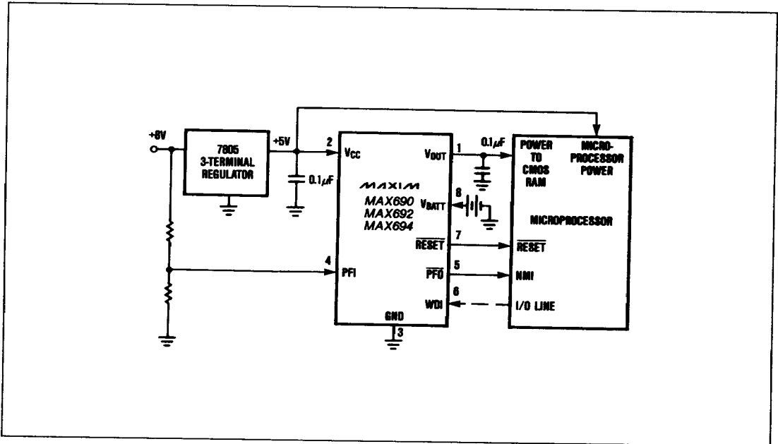
Figure 2. MAX690/692/694 Typical Application
