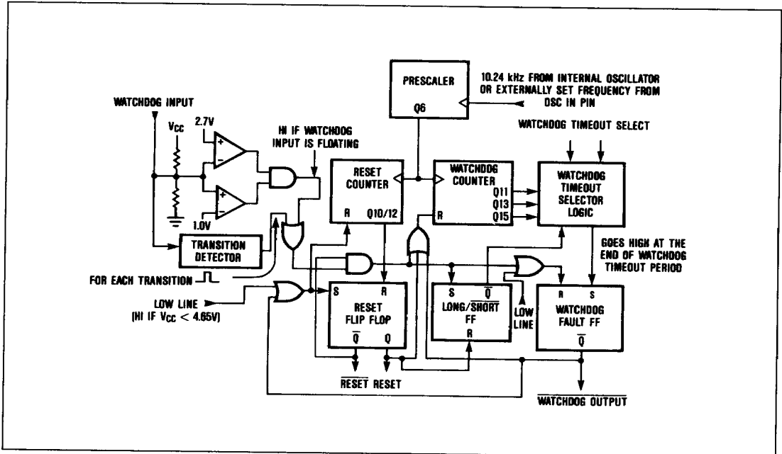
Figure 7. Watchdog Timer Block Diagram
